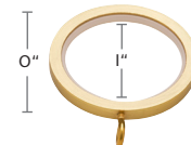
3035RIN-XX 1 3/8" Flat Ring w/ Plastic Insert O: 2 1/2" I: 1 7/8"
