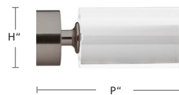
3045CIL-XX 1 3/4" Cylinder Finial H: 2 1/4" P: 5 1/8"
