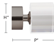
3045PIL-XX 1 3/4" Pillbox Finial H: 2 3/4" P: 3 1/2"
