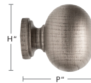
1145OVA-5X 1 3/4" Oval Ball Finial H: 3 1/2" P: 3 3/8"
