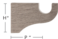
1235WBR-5X 1 3/8" Wall Bracket H: 3 3/8" P: 3 3/4" 1245WBR-5X 1 3/4" Wall Bracket H: 3 3/8" P: 3 3/4"
