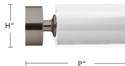
3035CIL-XX 1 3/8" Cylinder Finial H: 1 3/4" P: 4 1/4" 3045CIL-XX 1 3/4" Cylinder Finial H: 2 1/4" P: 5 1/8"
