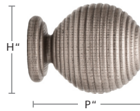
1135GRO-5X 1 3/8" Grooved Finial H: 2 3/4" P: 3 5/8" 1145GRO-5X 1 3/4" Grooved Finial H: 3 1/4" P: 3 3/4"
