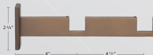
B11578-2-XX Berlin Double Wall Bracket
