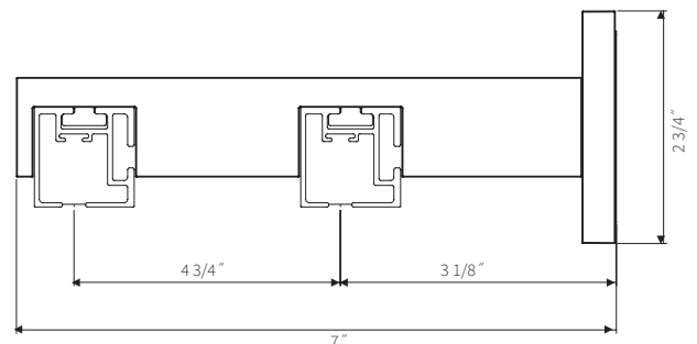
Double wall bracket 53410-XX
