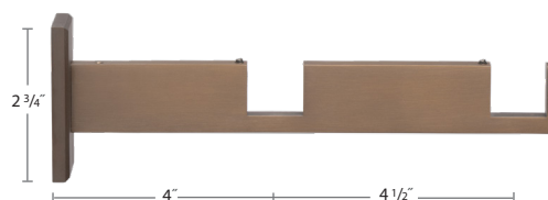
B11578-2-XX/XXX Berlin Double Wall Bracket
