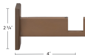
B11578-XX/XXX Berlin Single Wall Bracket
