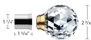
B3389-100 Ardea Finial B3389/1-XX Socket for Ardea Finial
