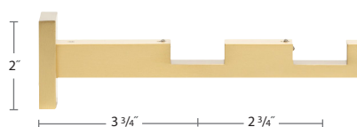
2230FDB-XX Faro Double Wall Bracket
