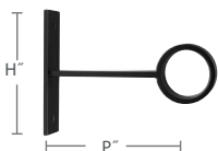
2220CYR-XX 3/4" York Single Closed Bracket H: 3 1/8" P: 3 1/4"
