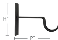
2220YOR-XX 3/4" York Single Open Bracket H: 3 1/8" P: 3 1/4"
