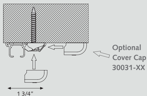
Heavy Duty Ceiling Bracket with Smart Klick 3003-XX
