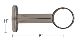
3035CWB-XX 1 3/8" Extended Closed Bracket H: 2" P: 3 1/2" (2 1/2" P also available)
