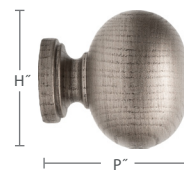
1135OVA-5X 1 3/8" Oval Ball Finial H: 3 1/4" P: 3 1/4"
