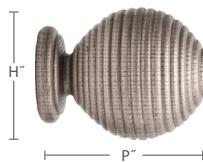
1135GRO-5X 1 3/8" Grooved Finial H: 2 3/4" P: 3 5/8"
