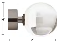
3035BAL-XX 1 3/8" Sphere Finial H: 2 3/8" P: 3 7/8" $229.05 ea. 3045BAL-XX 1 3/4" Sphere Finial H: 3" P: 4 3/4" $254.50 ea.
