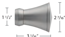
B610-XX Napoli Finial $530.59 ea.
