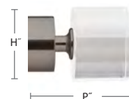
3035PIL-XX 1 3/8" Pillbox Finial H: 2 1/4" P: 2 3/4" $179.52 ea. 3045PIL-XX 1 3/4" Pillbox Finial H: 2 3/4" P: 3 1/2" $199.47 ea.
