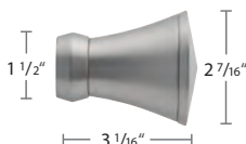
B610-XX Napoli Finial $530.59 ea.
