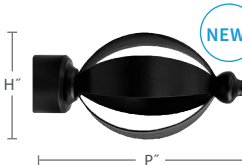
2120ROY-XX 3/4" Royal Finial H: 2 3/8" P: 4 7/8"
