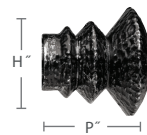
2120EVE-XX 3/4" Everest Finial H: 2" P: 1 7/8"
