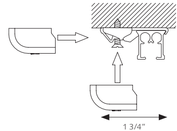
Smart Klick Ceiling Bracket with cover
