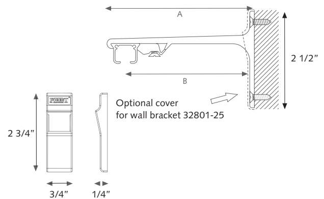
3" Single Wall Bracket 3280-XX
