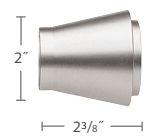
2130INC-XX Inca Finial
