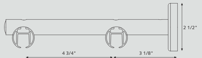
Extended Double Wall Bracket 53407-XX
