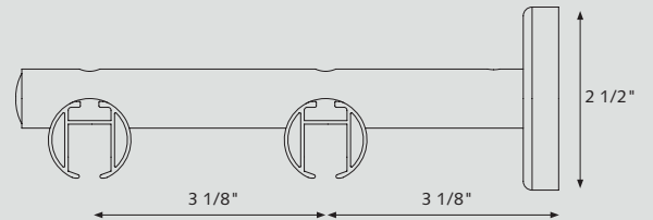
Double Wall Bracket 53406-XX
