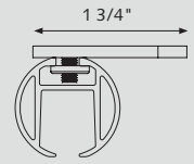
Flush Ceiling Bracket 53408-XX
